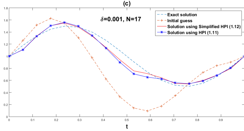
Fig. 3. Solution when N = 17 and \delta = 0.001
