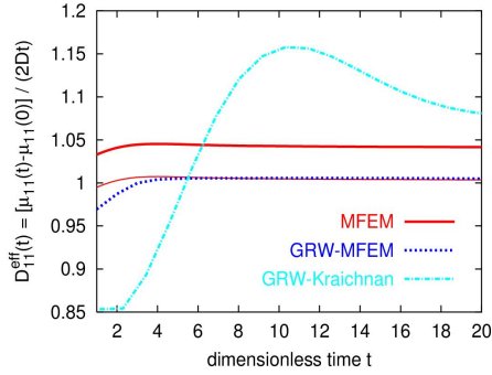
Figure 15: Longitudinal effective diffusion coefficients computed by full MFEM, coupled GRW-MFEM, and GRW-Kraichnan approximation.
