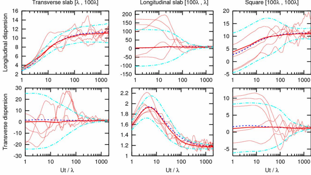
Figure 4: Single-realization dispersion (s_{ii} - S_{ii}(0))/(2Dt) (thin lines), one-particle dispersion X_{ii}/(2Dt) (dot lines), ensemble averages (S_{ii} - S_{ii}(0))/(2Dt) (thick lines), and (S_{ii} - S_{ii}(0) \pm SD(s_{ii}))/ (2Dt) (line-points).
