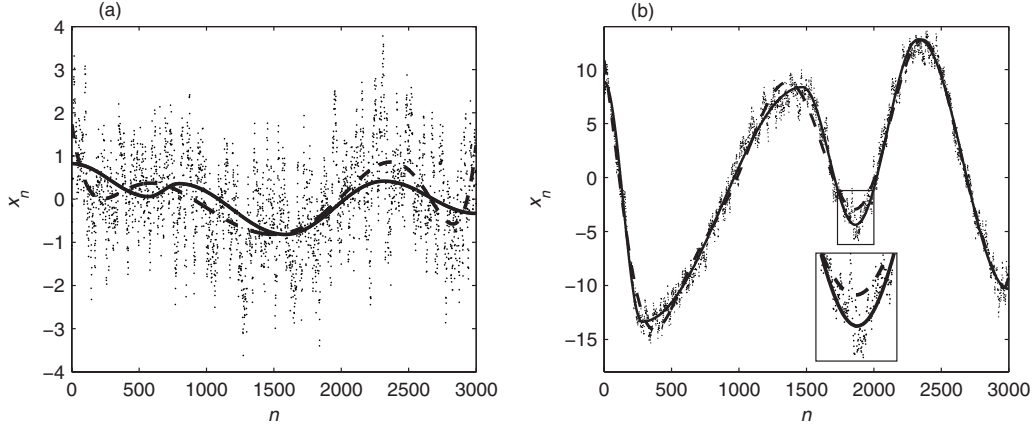
FIG. 2. Numerically generated trends obtained by superposing an AR(1) noise with \sigma=1 and \phi=0.9 over a deterministic trend (continuous line) composed by P=5 semiperiods of sinus with random lengths and amplitudes. The ratio between the amplitude of the trend and of the noise is r=0.25 (a) and r=4 (b). The dashed line is the estimated polynomial trend with the maximum resemblance with the real trend ( \eta minimum) but visually unacceptable due to local misfits, as in the zoom-in window.
