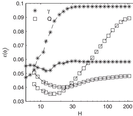
FIG. 8. The total errors of the estimated AR(5) parameters for the flickering time series in terms of the number H of the values of the serial correlation function used in calculations. The continuous line represents the error of \phi_1 and the dashed line that of \phi_5
