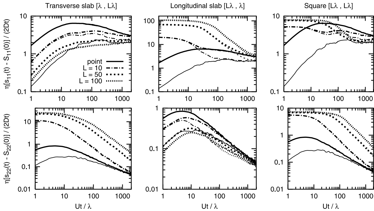
Figure 2. Ergodicity range \eta with respect to the memory-free dispersion and standard deviation SD(s_{II}) of the actual dispersion (thin lines) for different shapes and extensions of the initial plume.
