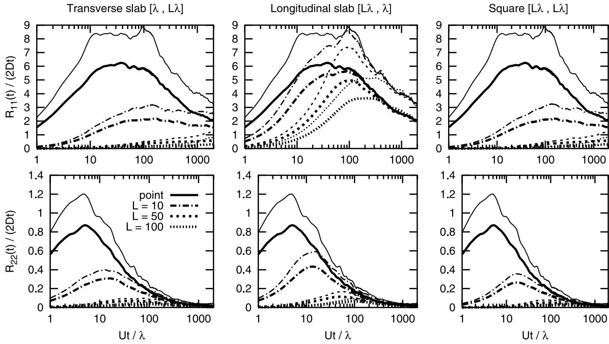
Figure 1. Variance of the plume center of mass R_{II} and corresponding standard deviation SD(r_{II}) (thin lines) for different shapes and extensions of the initial plume.
