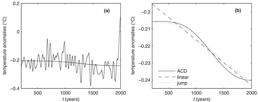
FIG. 8. Global mean annual temperature anomalies during the period A.D. 200–1995 with respect to the Northern Hemisphere mean annual temperature over 1856–1980 [9] and the trend estimated by means of ACD algorithm (continuous line). In panel (b) the trends estimated by means of the linear fit (dashed line) and jump process (dotted line) are also presented.
