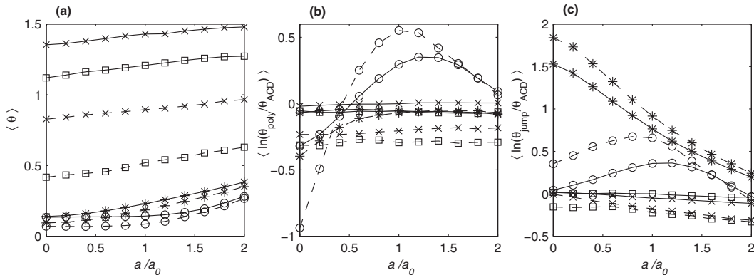
FIG. 13. (a) Dependence of the average evaluation index of the ACD algorithm on the parameter a in the trend formula f(t) = t + a \sin 2\pi t , t \in [0, 1] . The time series are characterized by different values of their length N and the random component of the signals is a stationary AR(1) noise with standard deviation \sigma_Z and different serial dependence \phi=0.9 (continuous lines) and \phi=0 (dashed lines). The couple (N, \sigma) takes the values (10,0.1) (asterisk marker *), (10,1) (cross marker ×), (50,0.1) (circle marker ○), and (50,1) (square marker □). A standard error smaller than 2% is obtained with statistical ensembles containing 1000 time series. (b) Comparison of the ACD accuracy with that of the linear fit for the same time series as for panel (a). (c) Comparison of the ACD accuracy with that of the jump process with R=0.4 and M=100 for the same time series as for panel (a).
