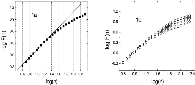
Fig. 1. (a) Detrended fluctuation analysis of AR(1) model for \varphi = 0.7 . A correlation exponent \alpha = 0.97 is calculated from the slope of straight line approximation of the first part of the plot. This correlation exponent is characteristic for the short range interval 0.6 < \log(n) < 1.4 . (b) The same plot generated with ten different random series.
