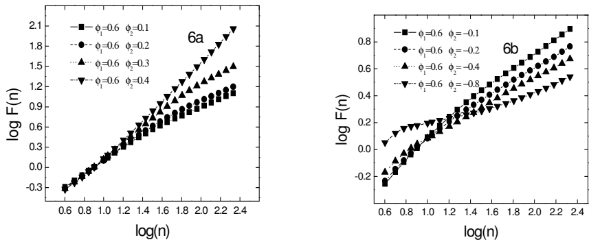
Fig. 6. (a) The influence of a positive value of \phi_2 on the DFA plot of an AR(2) model with \phi_1 = 0.6 . (b) The influence of a negative value of \phi_2 on the DFA plot of an AR(2) model with \phi_1 = 0.6 .
