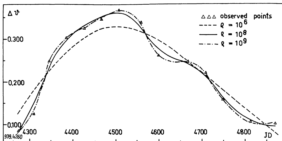
Fig. 1. Photoelectric observations of XZ Cyg made on 13 September 1973 and the smoothing spline-curves for q = 10^6 , 10^8 and 10^9 .
