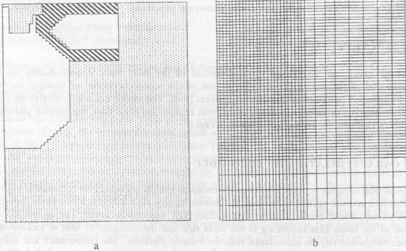
Fig. 1. The vertical section of spherical test (a) and its discretization network (b)
