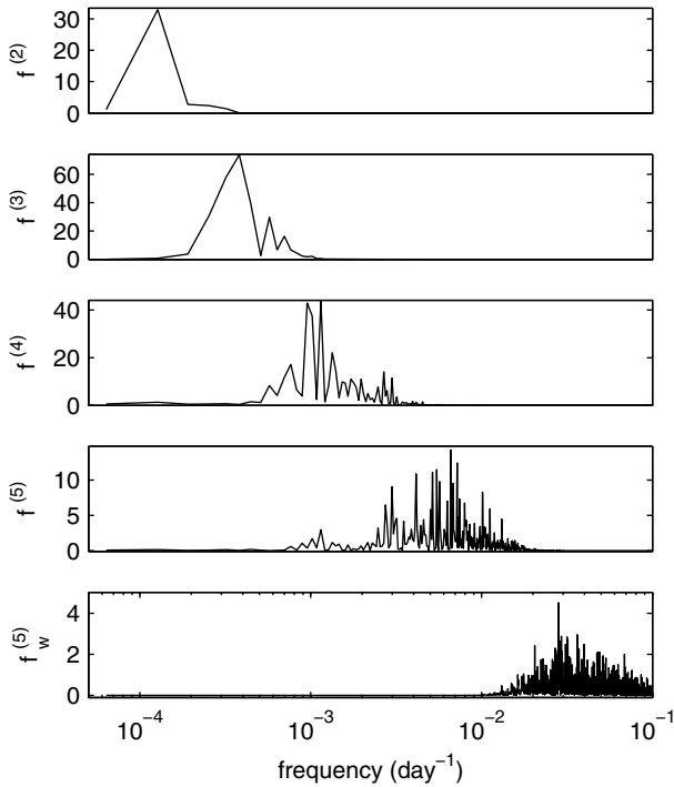
Fig. 5. The power spectra of the nonmonotonic intrinsic superstatistical components ( c > 1 ) and of the residuals of the estimated volatility of the S&P500 index.
