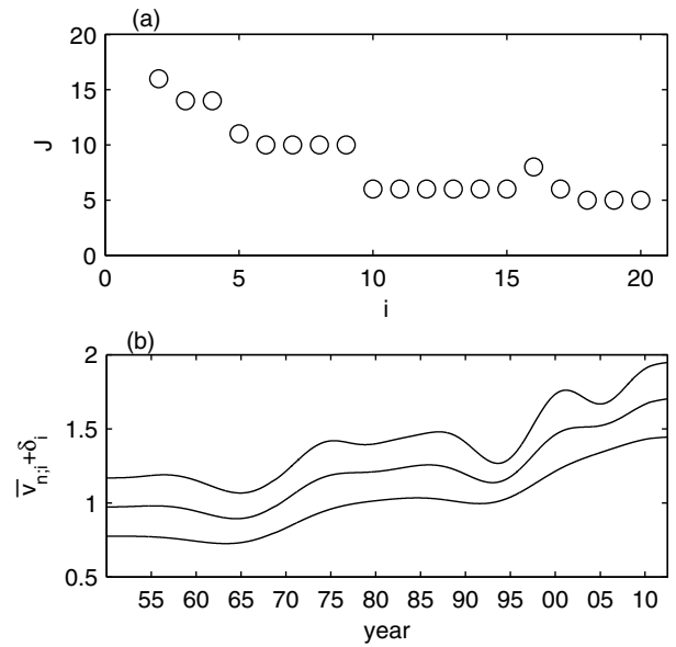
Fig. A.1. (a) The number of the monotonic segments of the averaged estimated volatility of the S&P500 index as a function of the number of averagings ( i > 1 ). (b) The estimated volatility averaged 6, 10, and 18 times. For clarity, the less smoothed time series are displaced by \delta_6 = 0.4 and \delta_{10} = 0.2 , while \delta_{18} = 0 .
