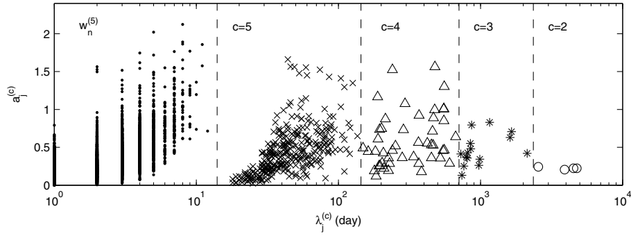
Fig. 4. The amplitude a_j^{(c)} equal with the overall variation of the j th monotonic segment of the c volatility intrinsic superstatistical component as a function of its characteristic time for the S&P500 index. The vertical dashed lines separate the disjoint intervals I_\lambda^{(c)} .
