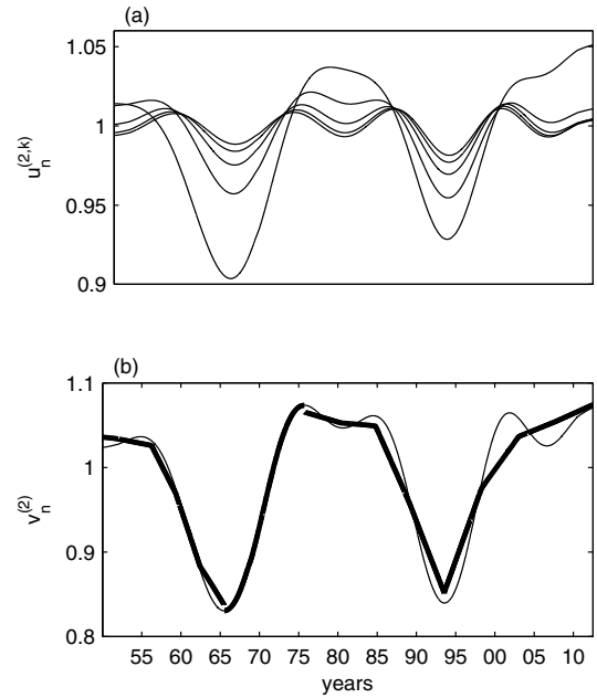
Fig. A.2. (a) The five partial averages u_n^{(2;k)} of the second intrinsic component of the S&P500 index. (b) The product of the first four partial averages (thin line) and the second intrinsic component (thick line) obtained after three applications of the ACD algorithm.
