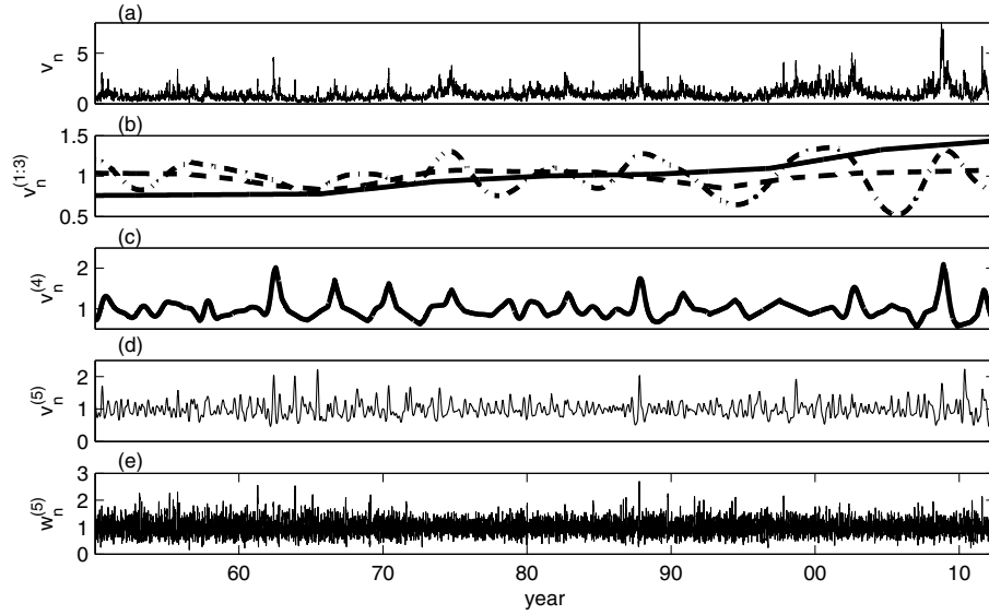
Fig. 3. (a) The estimated volatility of the S&P500 index divided by the mean volatility V . For a better visibility of the volatility shape, the range of the y-scale is reduced so that the maximum volatility occurring on 19 October 1987 is cut off. (b)–(e) The intrinsic superstatistical components and the residuals of the estimated volatility.
