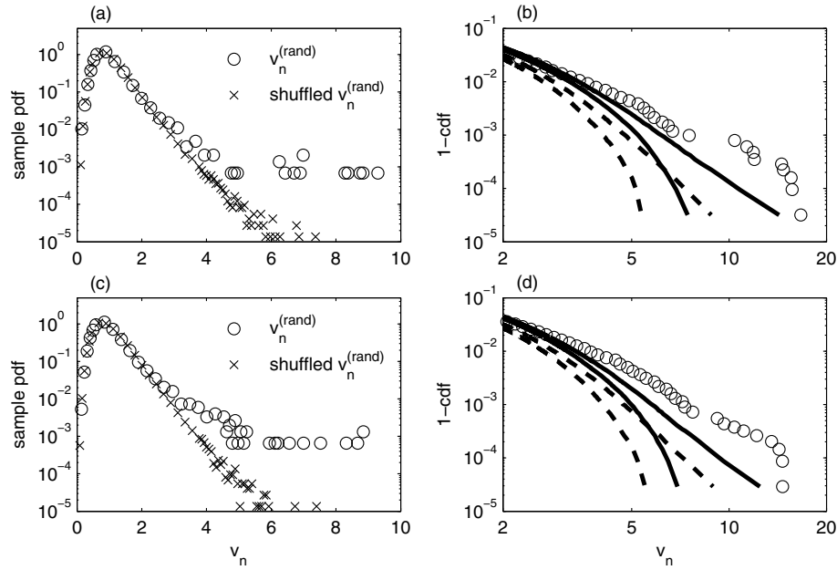
Fig. 7. The sample pdf of v_n^{(rand)} and of the product of the shuffled random intrinsic superstatistical components for the S&P500 index (a) and for the Nikkei index (c). The complementary cdf ( 1 - \text{cdf} ) of the standardized v_n^{(rand)} (circle markers) and the 95% interval of variation of the standardized product of the shuffled random intrinsic components (continuous lines) and of the Laplace distribution (dashed lines) for the S&P500 index (b) and for the Nikkei index (d).
